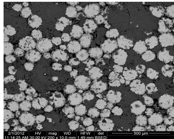
Fig. 10. SEM micrography of the composite with 70% 316L/ 30% Hap.
