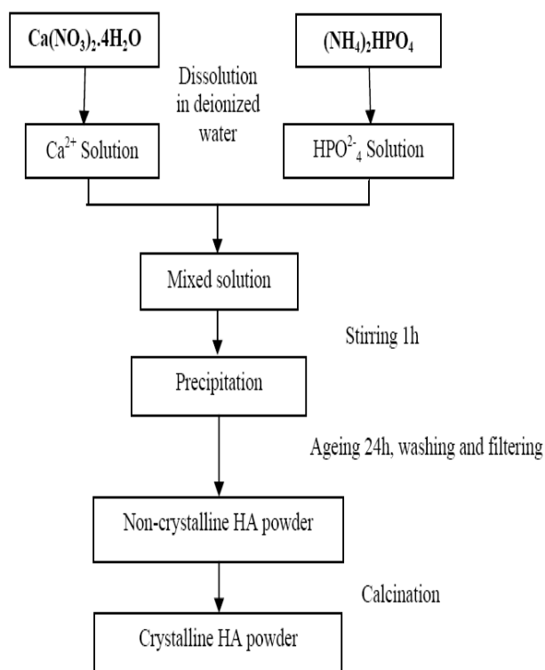
Fig. 1. Modified chemical precipitation route for HAP powder preparation. (Adapted from Sung)[3].
