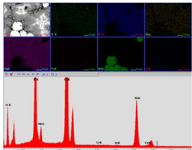
Fig. 11. EDAX for composit with 70% 316L and 30% HAP.
