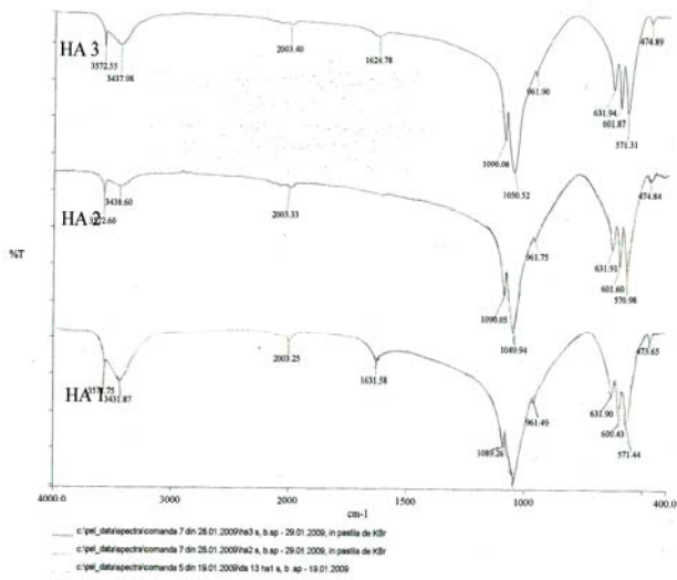
Fig. 2. FTIR analysis on the 3 HAp powders calcined at 800°C, 1000°C, 1200°C.
