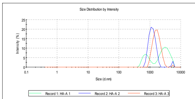
Fig. 3. Particle size distribution by intensity of the 3 records.
